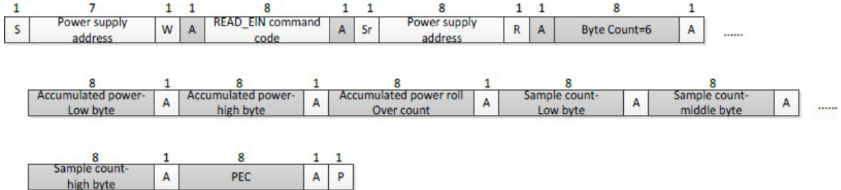
Figure 7 Read_EIN command
