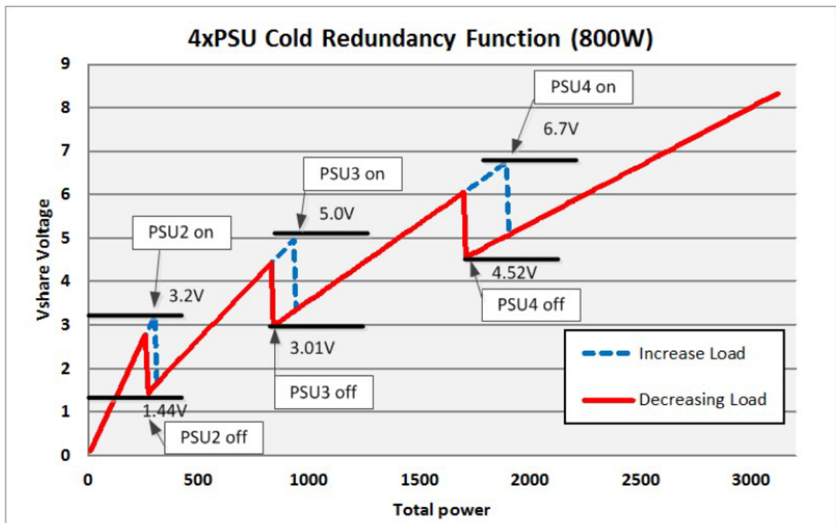
Figure 13 Example Power On/Off of power supplies in Cold Redundant Mode (4x1000W PSUs)
