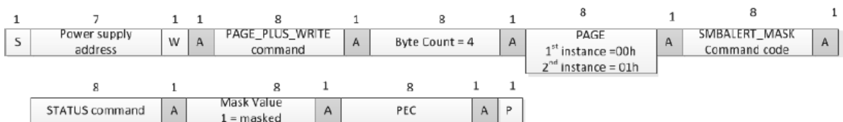
Figure 11 PAGE_PLUS_WRITE command.
