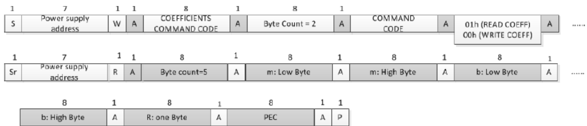
Figure 9 Retrieving Coefficients Using PEC
