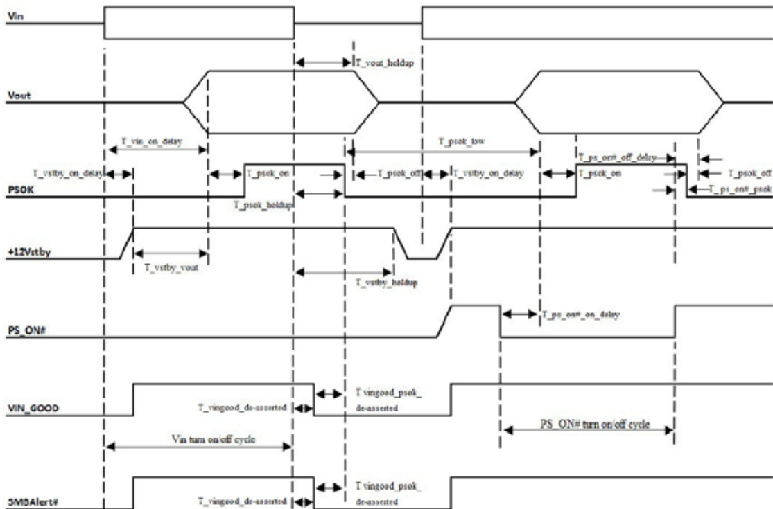
Figure 6 Turn On/Off Timing
