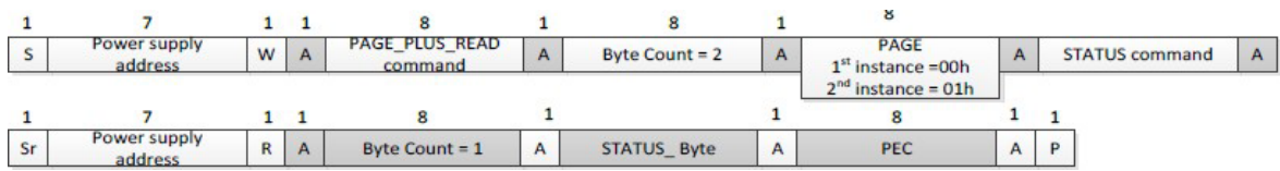
Figure 15 Reading STATUS Commands with PAGE_PLUS_READ
