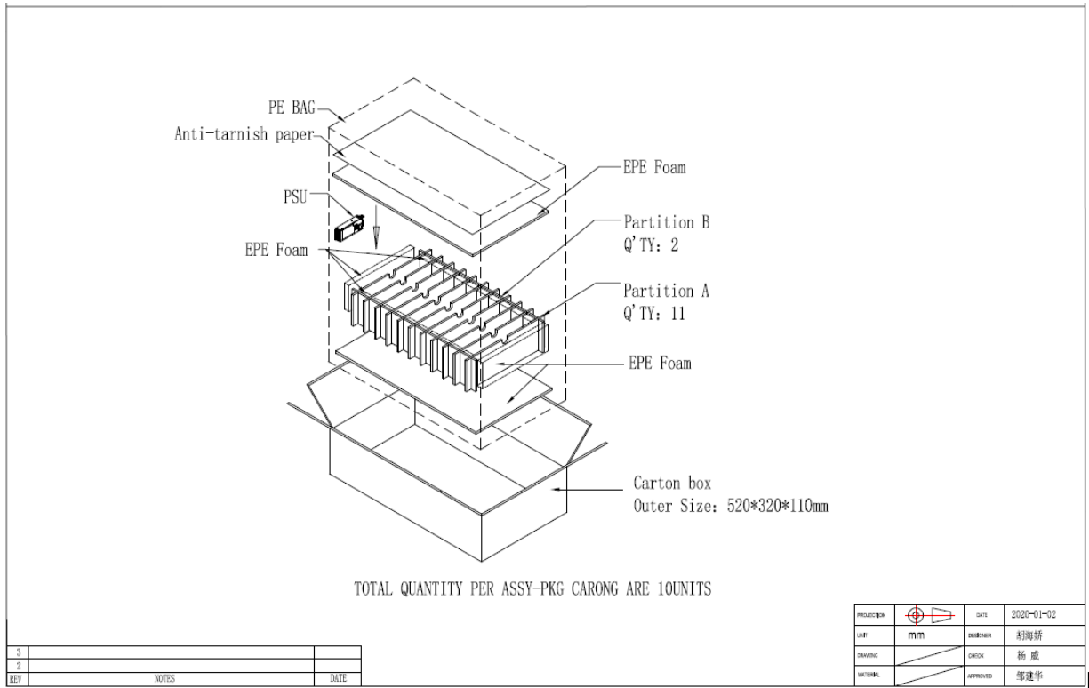
Figure 3 Packing Diagram
