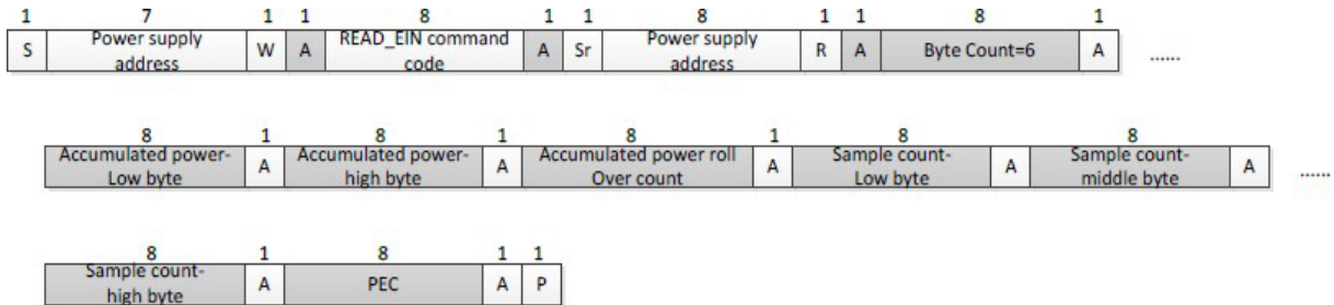
Figure 7 Read_EIN command
