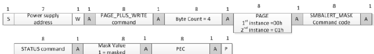
Figure 11 PAGE_PLUS_WRITE command.
